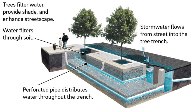
At Right: Graphic rendering of a completed stormwater tree trench similar to the one to be constructed along Fairmount Avenue between N. Uber Street and N. 19 th Street
