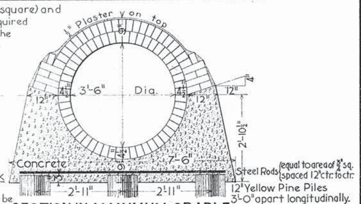
SECTION IN MAXIMUM CRADLE
