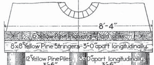
SECTION SHOWING PLATFORM AND PILES
