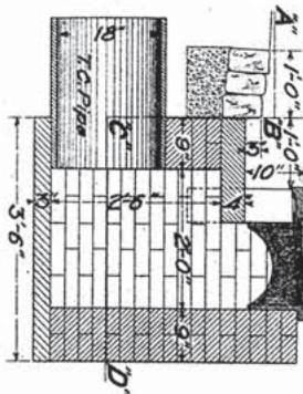
SECTION E-F
