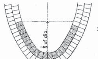
VITRIFIED SHALE BRICK INVERT
