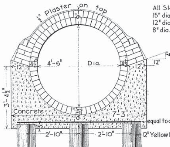
SECTION IN REDUCED GRADE
