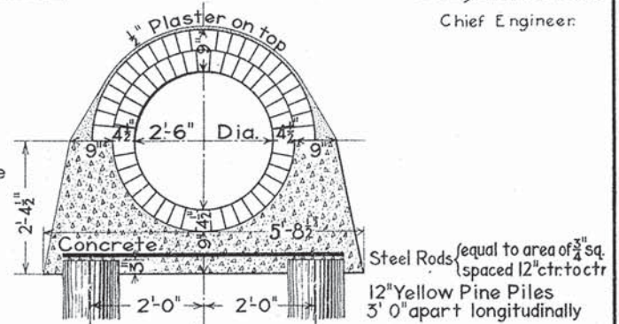
SECTION IN MAXIMUM CRADLE
