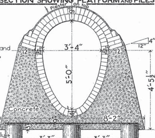
SECTION IN MAXIMUM CRADLE
