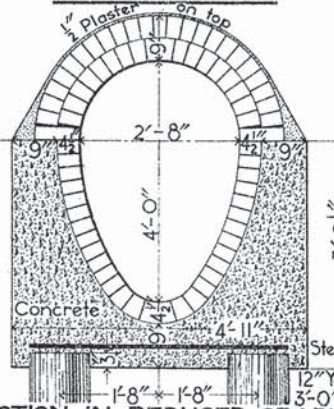
SECTION IN REDUCED CRADLE
