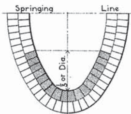
SECTION IN MAXIMUM CRADLE
