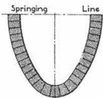
SECTION IN MAXIMUM CRADLE
