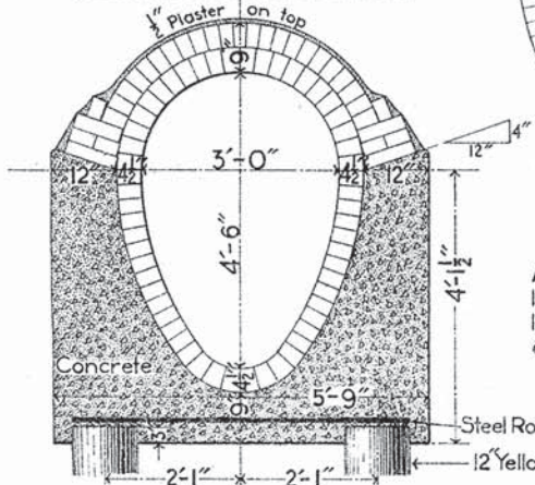
SECTION IN REDUCED CRADLE
