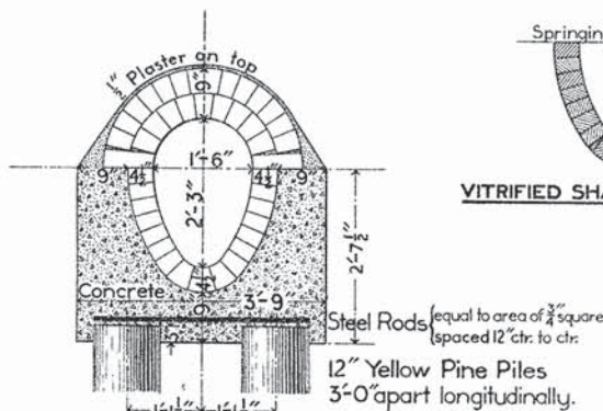
SECTION IN REDUCED CRADLE
