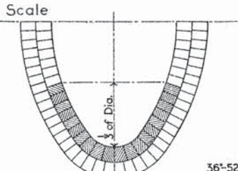
VITRIFIED SHALE BRICK INVERT
