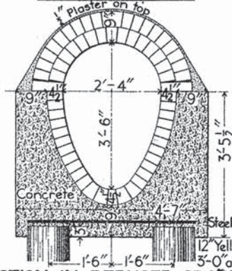
SECTION IN REDUCED CRADLE
