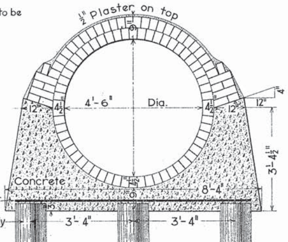
SECTION IN MAXIMUM GRADE
