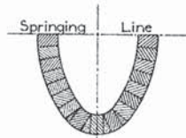
VITRIFIED SHALE BRICK INVERT.
