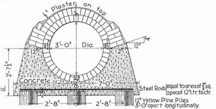
SECTION IN MAXIMUM CRADLE
