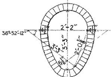
MINIMUM SECTION
