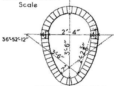
MINIMUM SECTION
