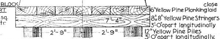
SECTION SHOWING PLATFORM and PILES
