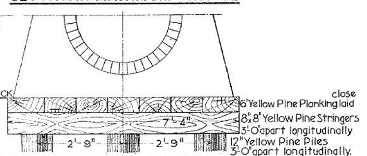
SECTION SHOWING PLATFORM and PILES
