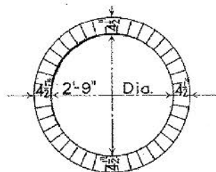
MINIMUM SECTION
