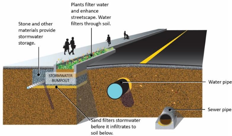
At Right: Graphic rendering of completed work at 64th Street near City Avenue (SR 0001).
