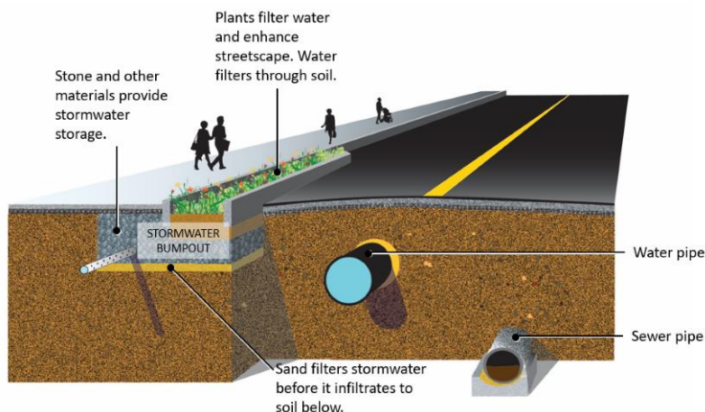
At Right: Graphic rendering of a completed stormwater bumpout at 66 th Street and Guyer Avenue.
