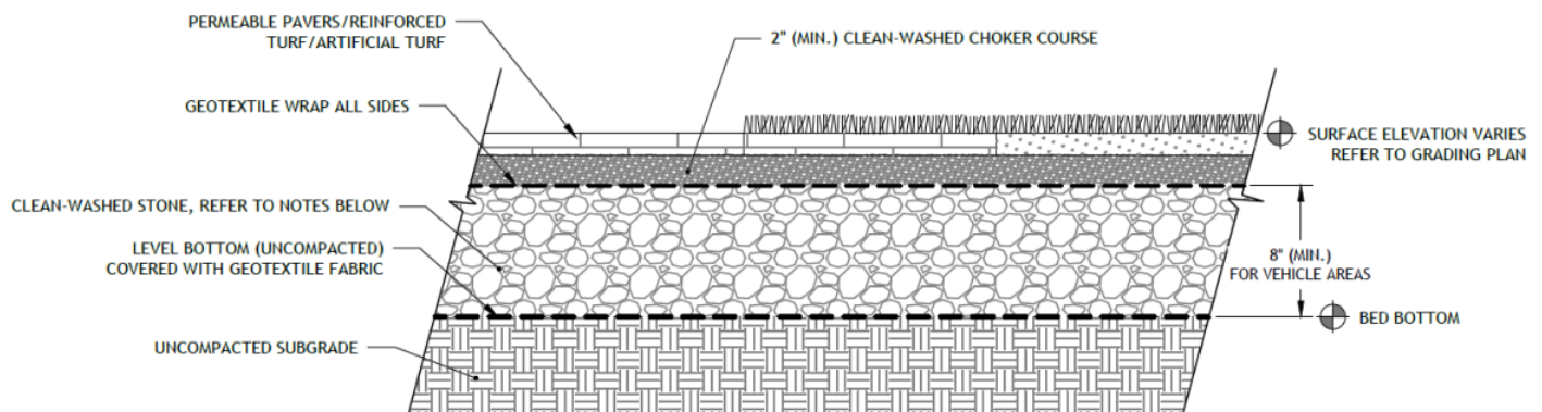
Figure 4.2-3: Terraced porous surfaces standard detail
