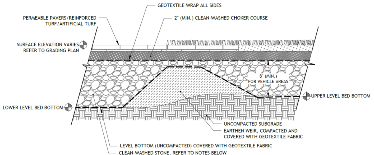
Figure 4.2-3: Terraced porous surfaces standard detail
