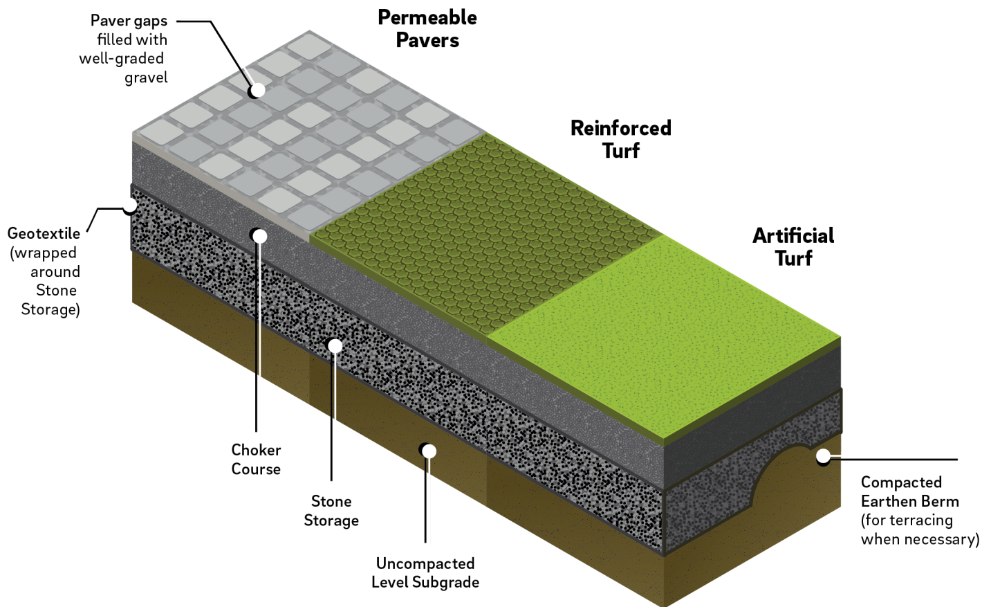
Figure 4.2-1: Porous surfaces with typical features
