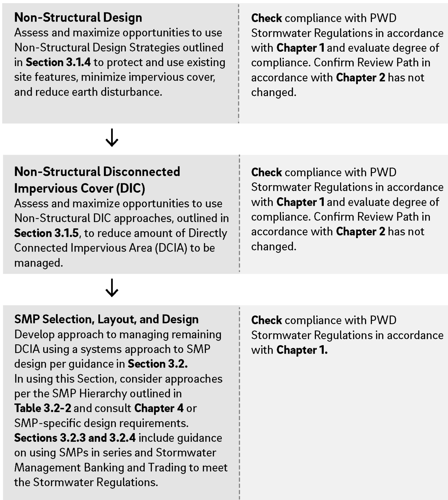
Figure 3.1-1: PWD's Integrated Design Approach
