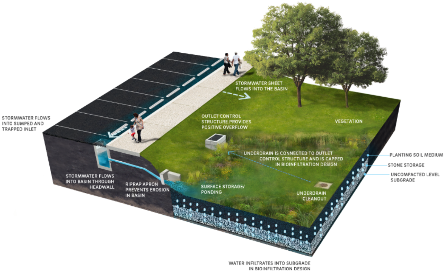
Figure 4.1-1: Bioinfiltration/Bioretention Basin with Typical Features
