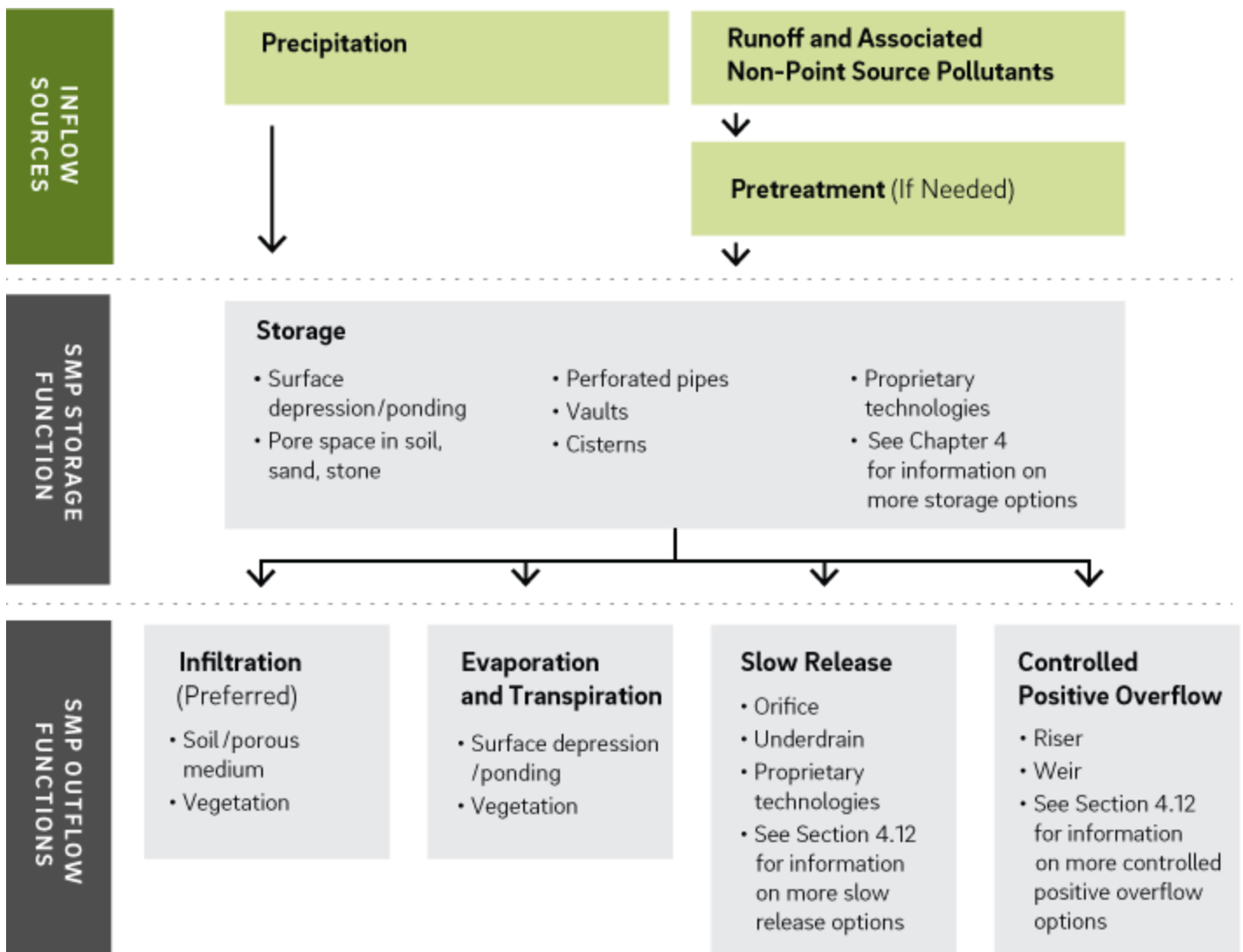
Figure 3.1-3: Overview of SMP Functions
