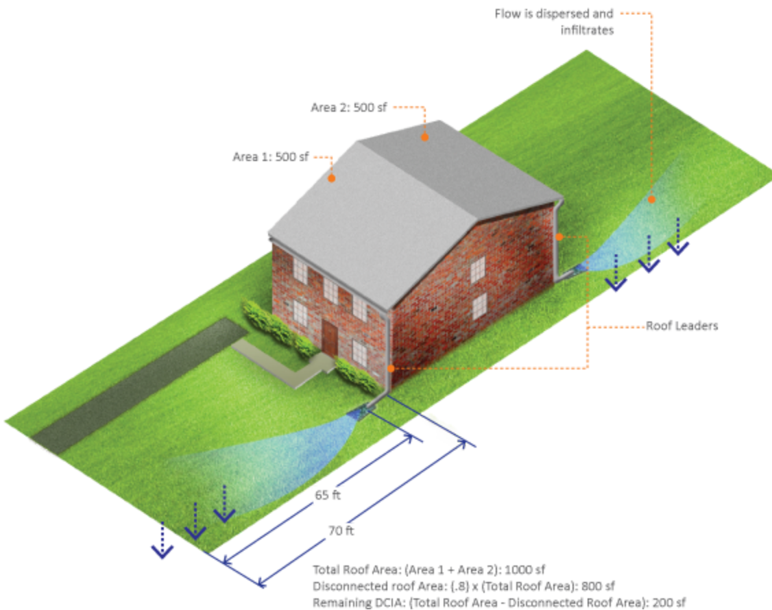
Figure 3.1-2: Rooftop Disconnection Example
