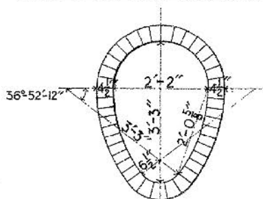
MINIMUM SECTION
