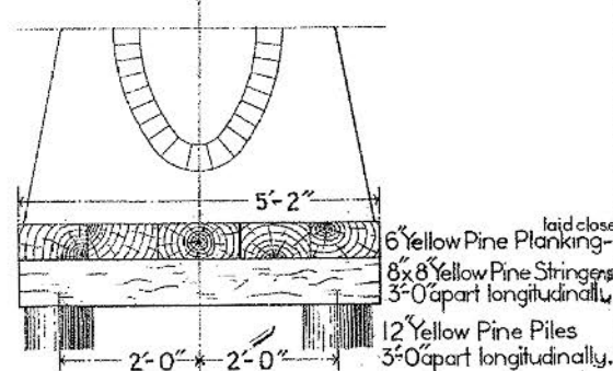
SECTION SHOWING PLATFORM AND PILES
