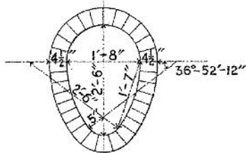
MINIMUM SECTION
