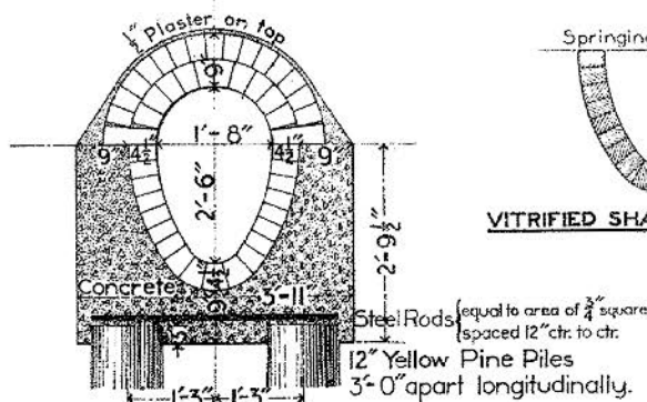
SECTION IN REDUCED CRADLE
