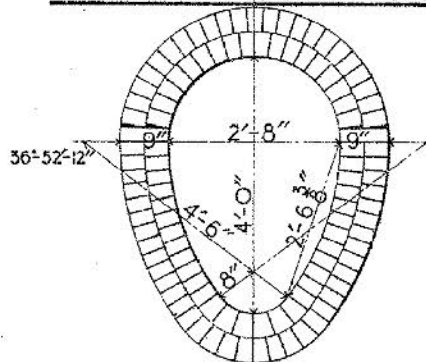
MINIMUM SECTION
