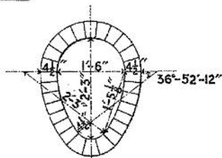
MINIMUM SECTION
