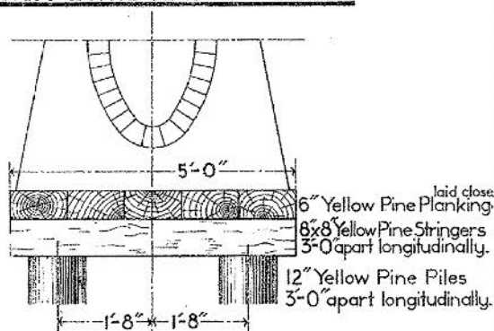
SECTION IN MAXIMUM CRADLE
