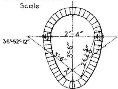
MINIMUM SECTION
