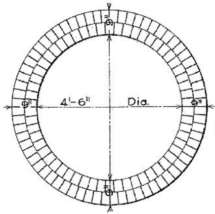
MINIMUM SECTION
