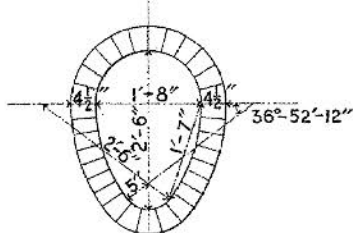
MINIMUM SECTION
