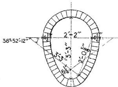
MINIMUM SECTION
