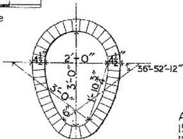
MINIMUM SECTION
