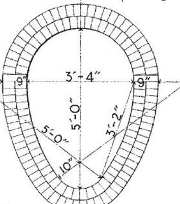
MINIMUM SECTION
