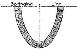
VITRIFIED SHALE BRICK INVERT
