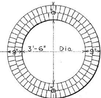
MINIMUM SECTION
