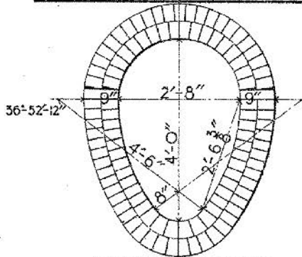
MINIMUM SECTION
