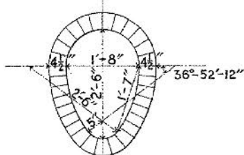
MINIMUM SECTION
