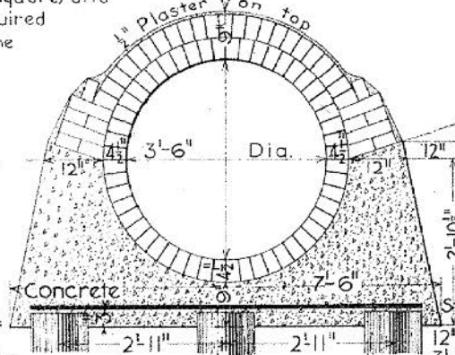
SECTION IN MAXIMUM CRADLE
