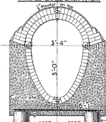
MINIMUM SECTION
