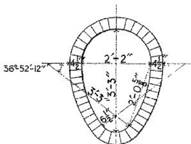
MINIMUM SECTION
